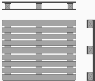
CP1 1000 × 1200 mm
