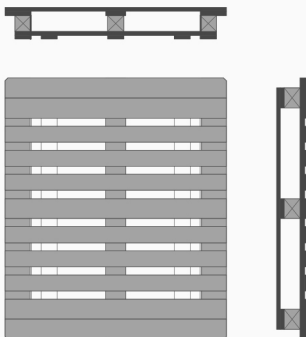
CP7 1300 × 1100 mm
