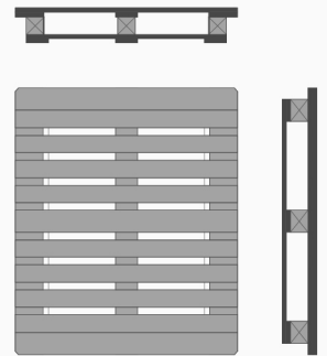
CP6 1200 × 1000 mm
