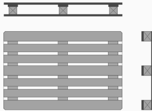
CP2 800 × 1200 mm
